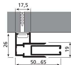
Face Fix Side Channel
