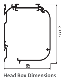
Head Box Dimensions
