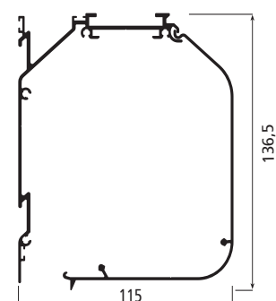
Side Fix Side Channel
