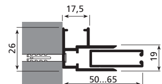
Side Fix Side Channel
